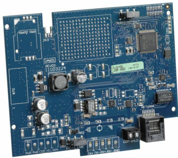
TL280LER-AT PowerSeries NEO dual path LTE/IP Alarm Communicator
