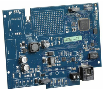
TL280LE-AT PowerSeries NEO Dual Path LTE-IP Alarm Communicator
