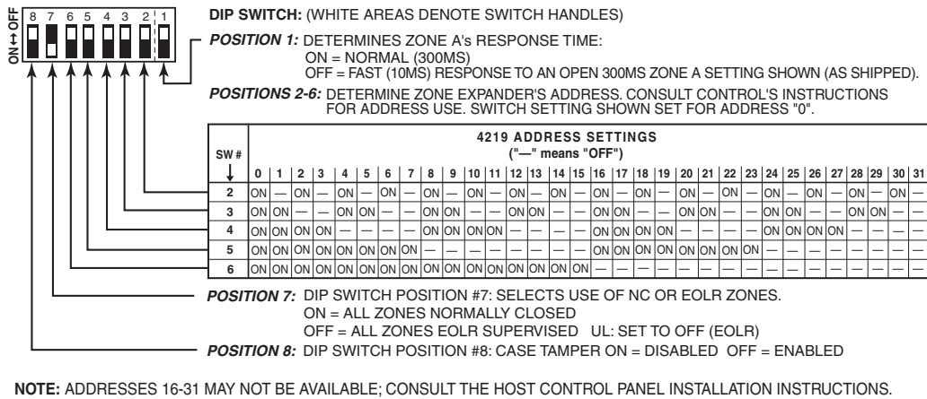
Figure 3. DIP Switch Settings
