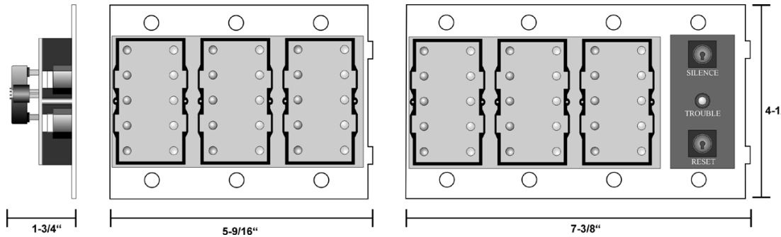
5865-3 and 5865-4 Dimensions
