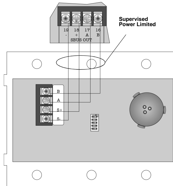
Figure 1: 5865-3 or 5864-4 Connection to the 5820
