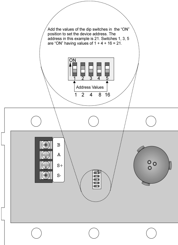
Figure 2: Setting the Device Address
