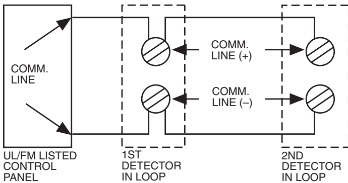
FIGURE 6. SYSTEM WIRING DIAGRAM FOR SK-DUCT-W
